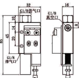
CV-10HSCK带信号开关
