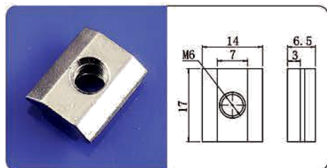
M6凸形单孔螺母
