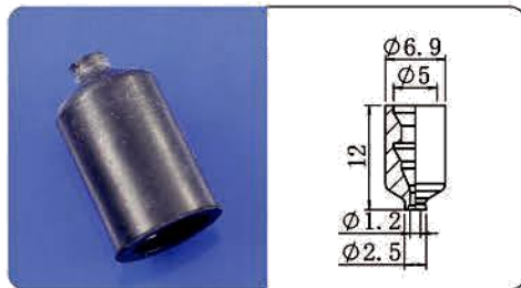
CP-02UN
