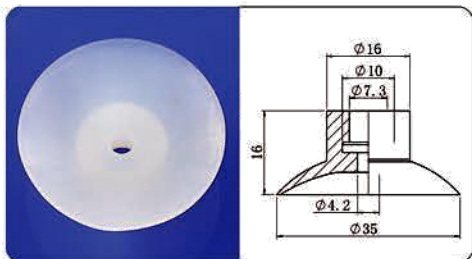
HSP-35
