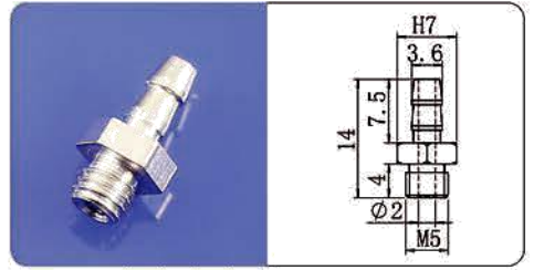
M5-4二节气咀
