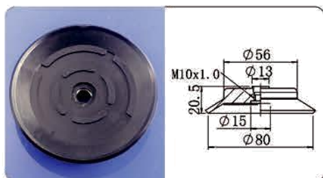
PF-80N
