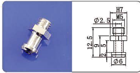
SPPS-M5 B
