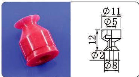
SR-8
