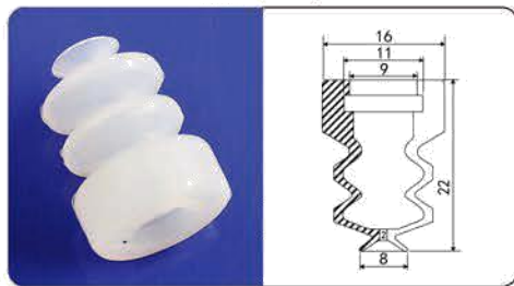
YX-8-3S
