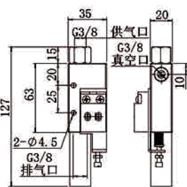
CV-15HSCK带信号开关
