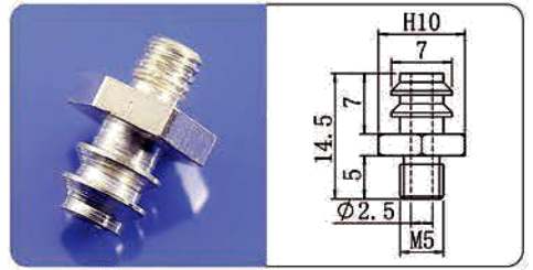
M5-7二节气咀
