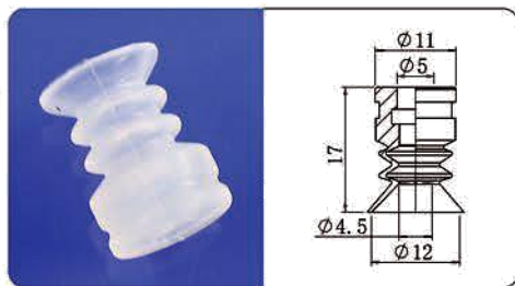
SR-12-3S
