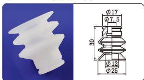
SR-25-3S
