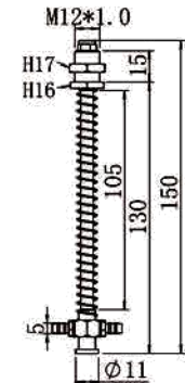
TL-M12-L150-11
