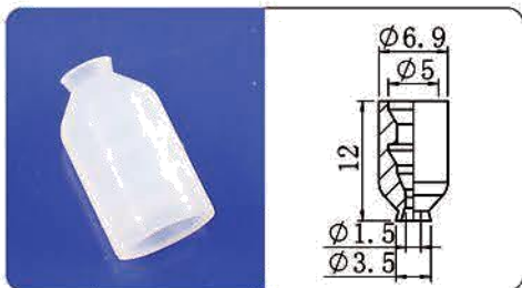
CP-03U
