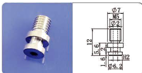
转换头P6M5N
