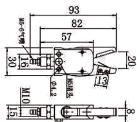
Mini-A外牙带检知
