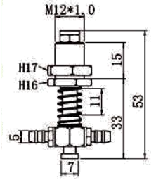
TL-M12-L53-7
