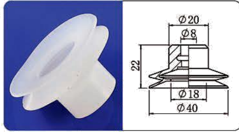
HSP-40-2
