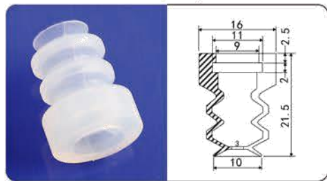
YX-10-3S
