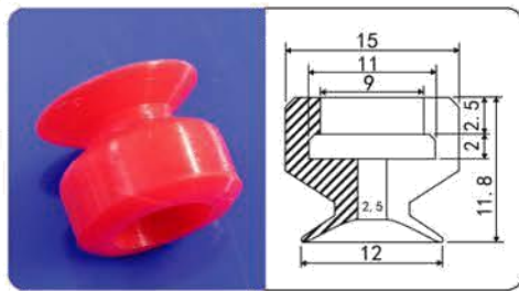
YX-12R
