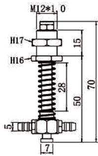
TL-M12-L70-7
