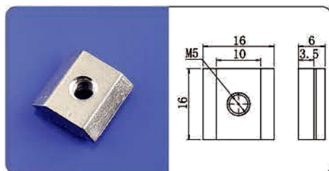
凸形单孔螺母M5
