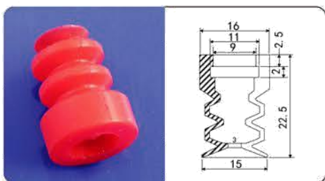
YX-15-3R
