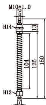
TS-M10-L150-7
