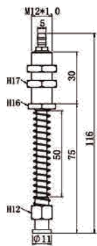
TS-M12-L116-11B
