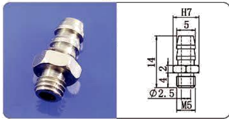
M5-6二节气咀
