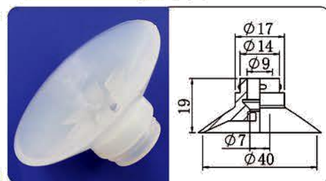
CP-40C
