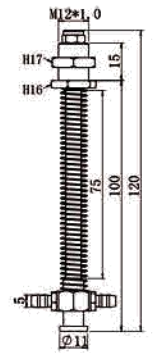
TL-M12-L120-11
