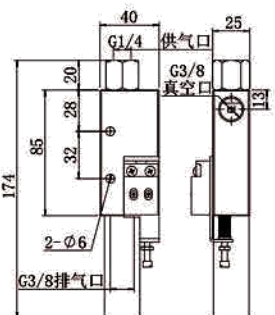
CV-20HSCK带信号开关
