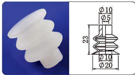
PC-20
