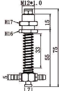
TL-M12-L75-7
