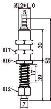
TS-M12-L80-7B
