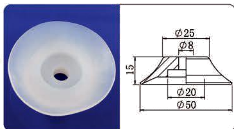
PF-50
