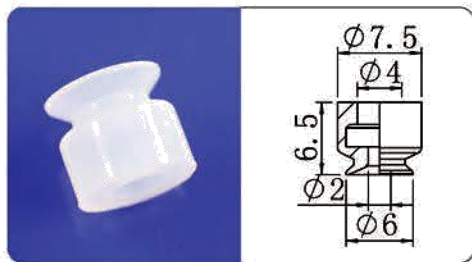
PF-6
