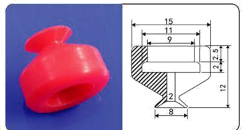
YX-8R
