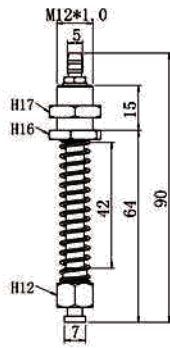
TS-M12-L90-7
